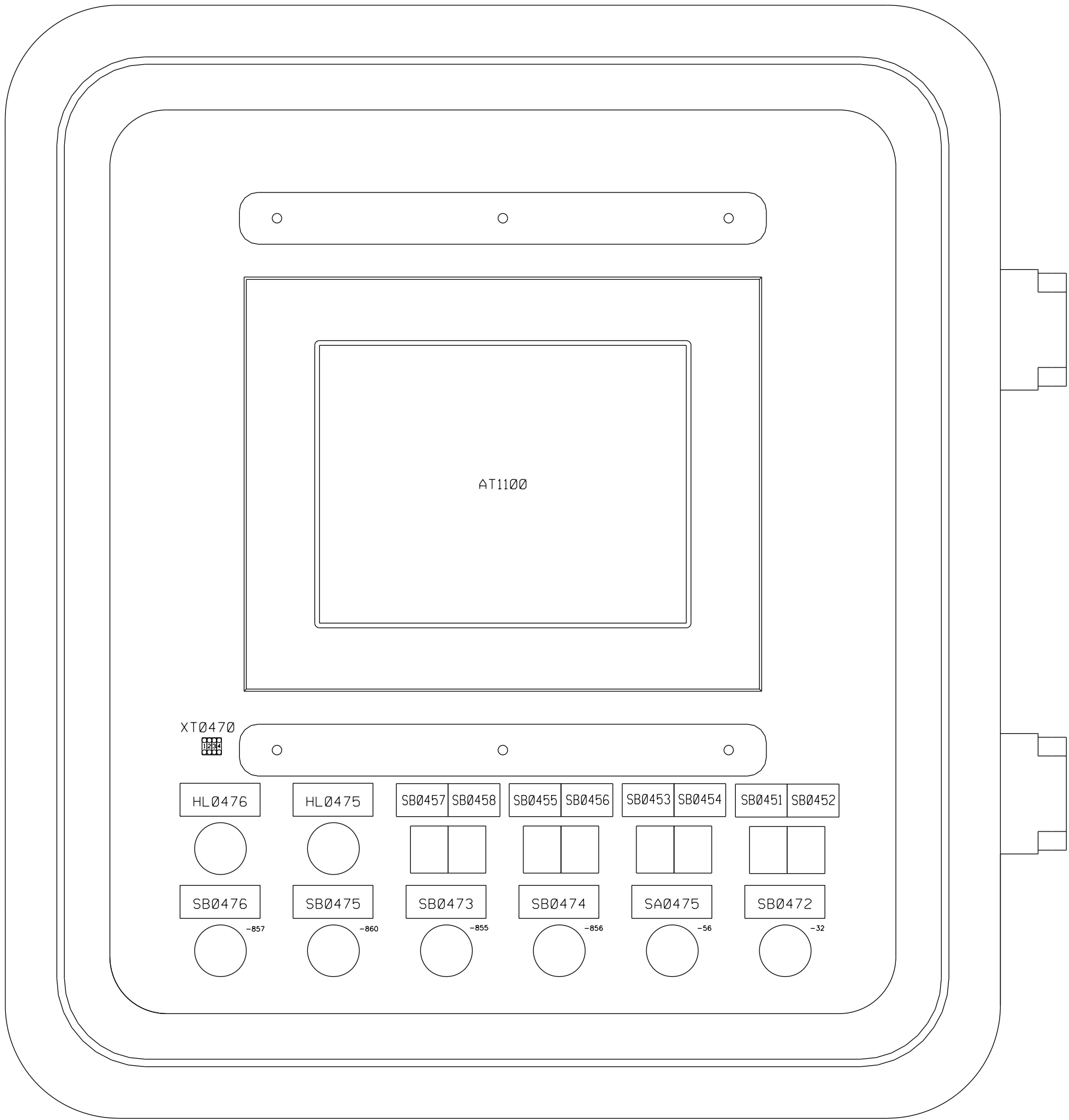
COVER Open
